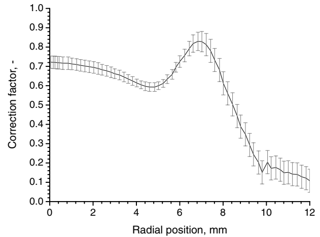
Fig. 8 Computed correction factor profile; P = 300 mbar.
