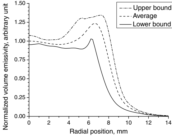
Fig. 4 Envelope and average value of the Abel-inverted emission fluctuations at P = 300 mbar, optimized geometry.
